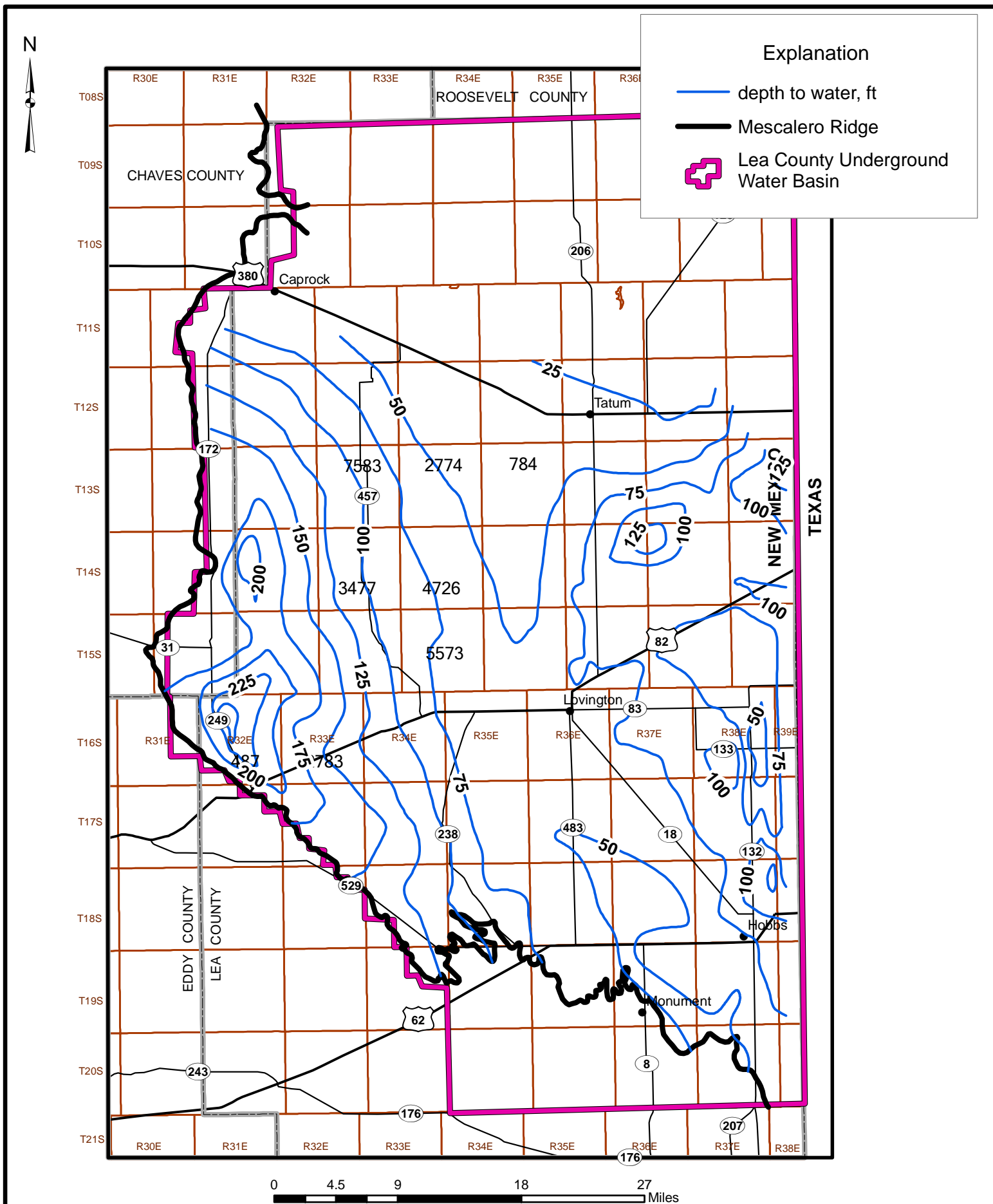
Figure 6. Map showing depth to water based on data from 2001 to 2008 in the Ogallala aquifer in the Lea County Underground Water Basin.
