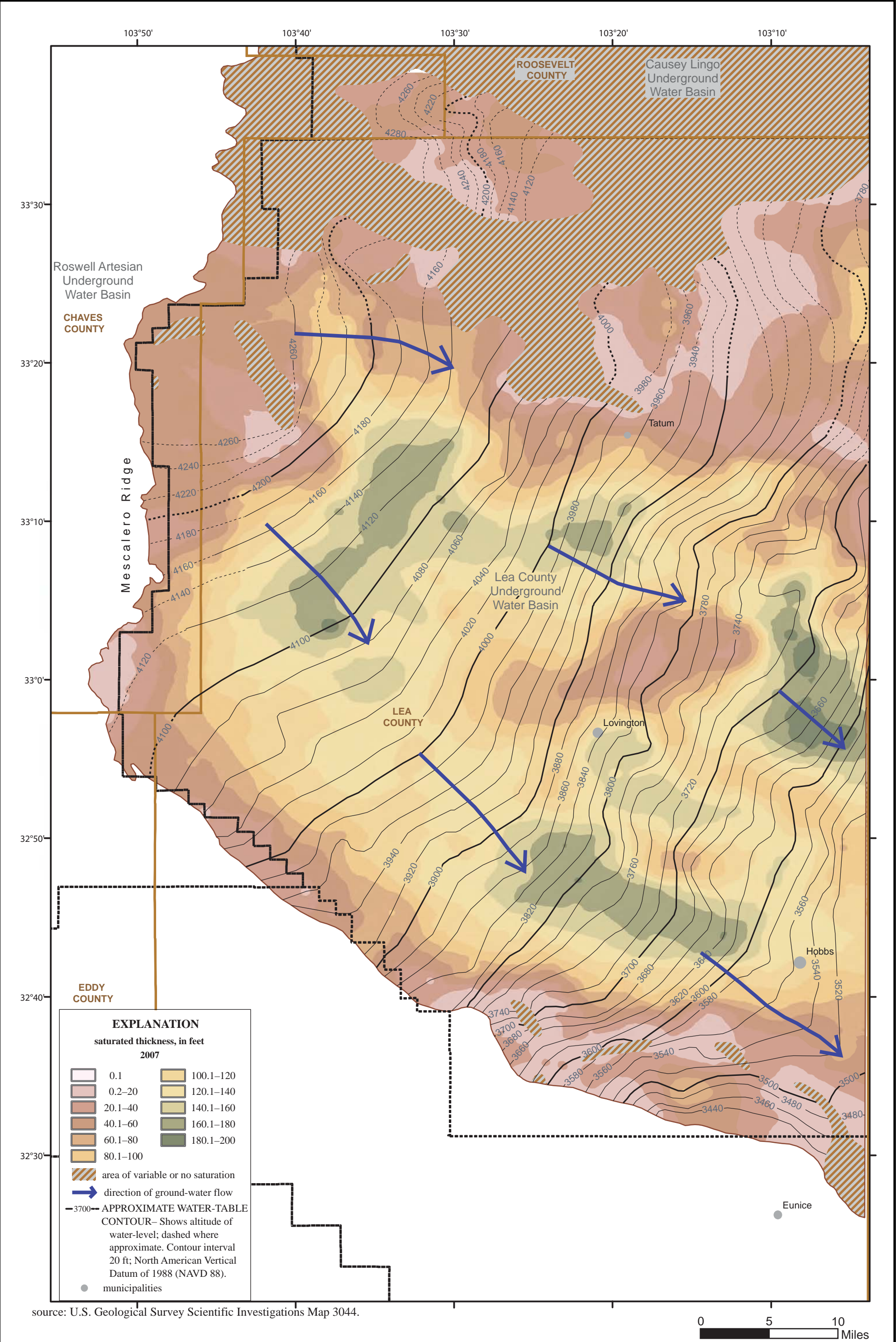
Figure 7. Map showing water-table contours, saturated thickness, and direction of groundwater-flow, based on 2004 to 2007 groundwater-level data measurements of the Ogallala aquifer in Lea County Underground Water Basin.
