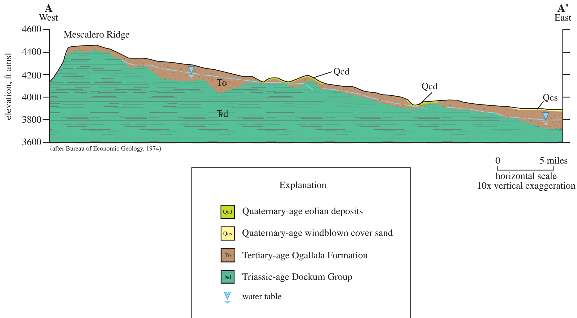
Figure 4. Geologic cross-section A-A', Lea County, New Mexico. See Figure 3 for line of section.
