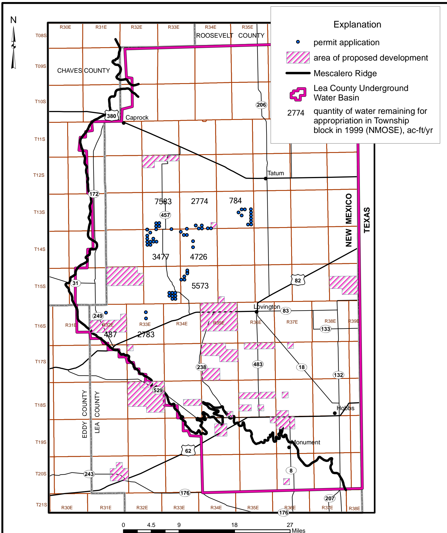
Figure 1. Map showing Lea County Underground Water Basin, permit application locations, quantity of water remaining in Township block, and areas of proposed development where water will be put to beneficial use, Lea County, New Mexico.
